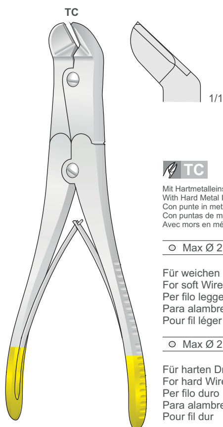
LX-105 230 mm
